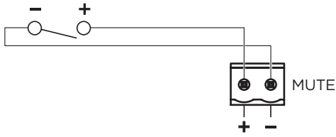
Figure 16. Amplifier mute contact closure
